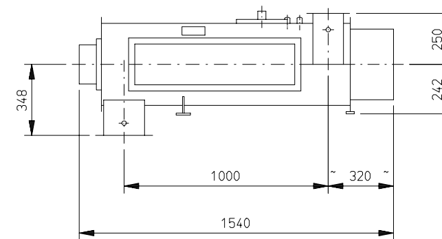
CONDITIONER 400X1200
